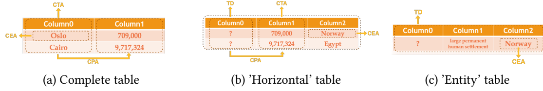
Figure 1: SemTab tasks
