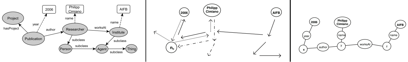
Fig. 3. a) Augmented Summary Graph b) Exploration c) Query Mapping
