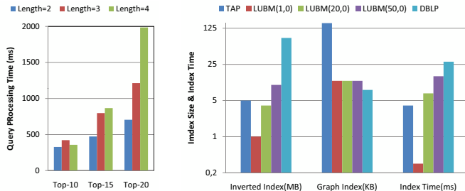
Fig. 6. a) Query Performance b) Index Performance
