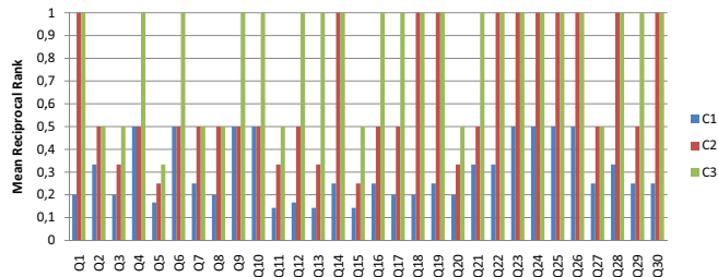
Fig. 4. MRRs of different Scoring Functions on DBLP
