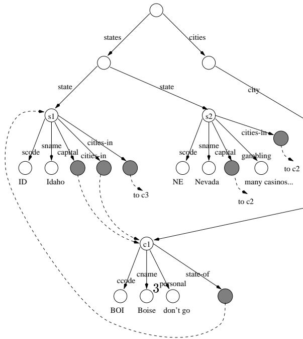
Figure 1: Some (rather regular) XML data
