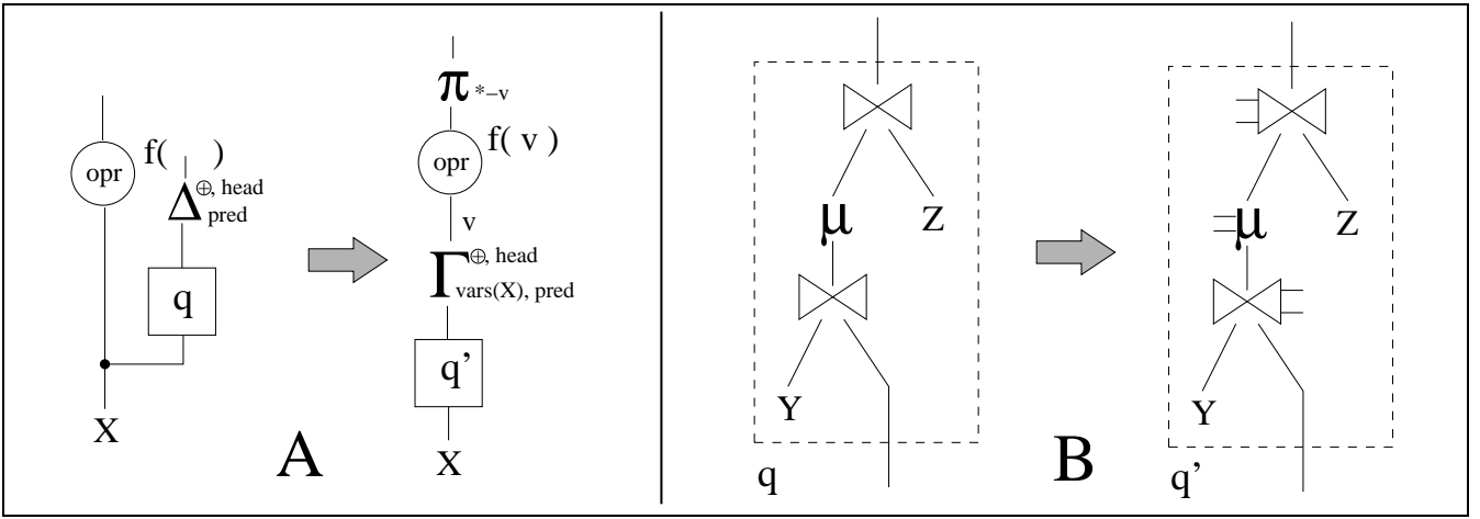
Figure 2: Algebraic Query Unnesting
