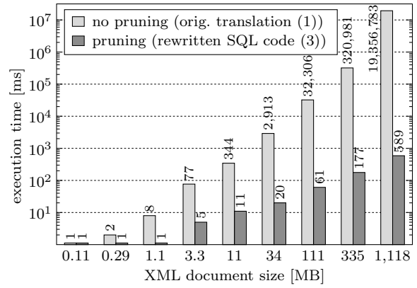
Figure 11: Context set pruning speeds up the evaluation of /descendant::city/following::zipcode by orders of magnitude.
