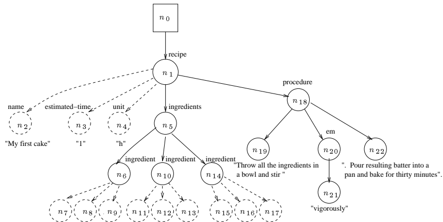
Fig. 2. The tree corresponding to the recipe document in Fig. 1. Some details are omitted. For example, the nodes n_7 , n_8 , and n_9 are the attribute nodes named quantity, unit, and name of the first ingredient.
