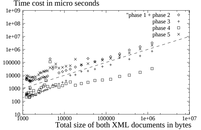
Figure 4. Time cost for the different phases
