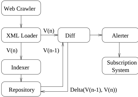
Figure 1. Xyleme-Change architecture
