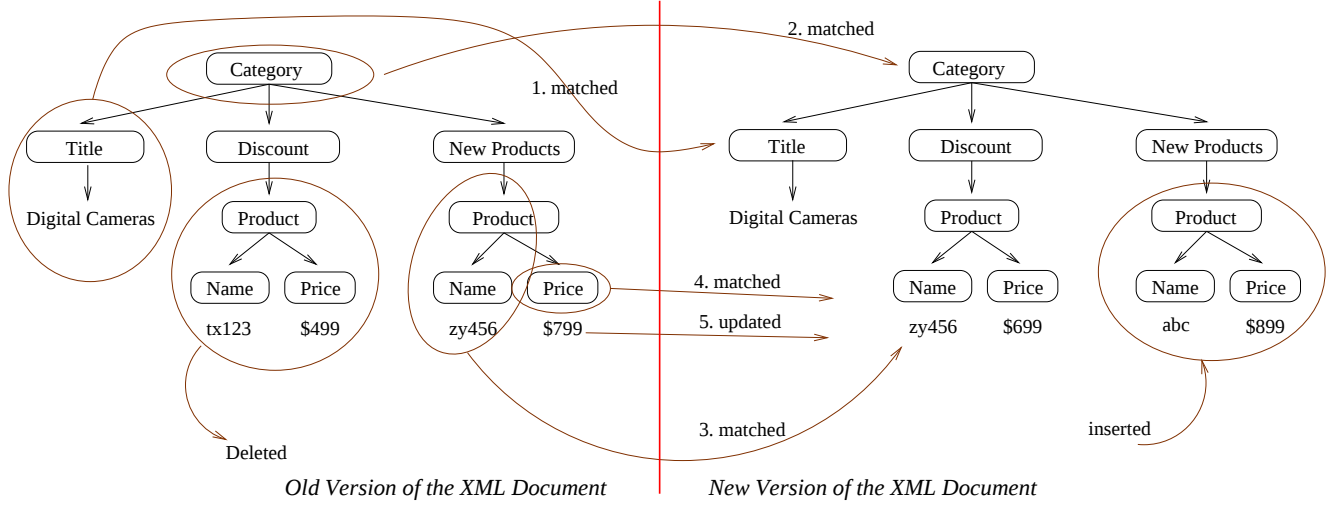
Figure 2. Matching subtrees
