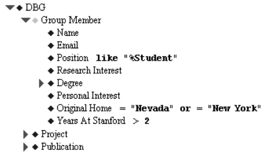
Figure 9. A DataGuide query specification
