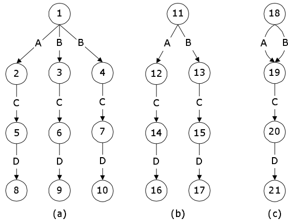
Figure 3. A source and two DataGuides
