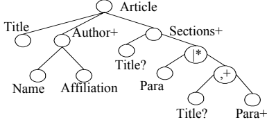
Figure 3. DTD tree for the DTD in Figure 2.
