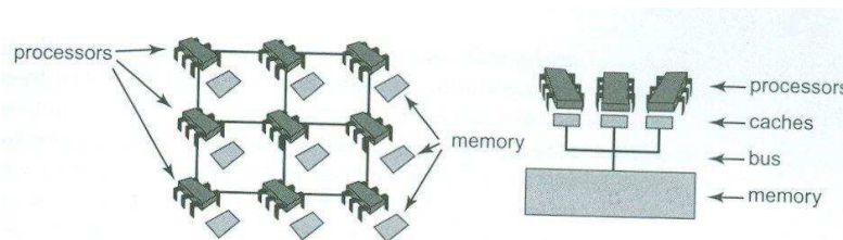
Cache-less NUMA architecture
