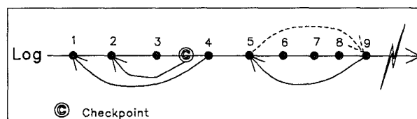
Fig. 18. Partial rollback handling in System R.
