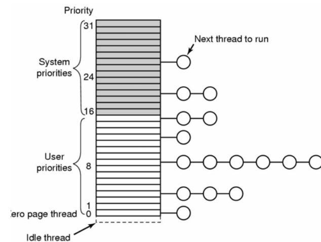
Windows 2000 supports 32 priorities for threads
