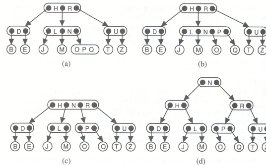
Σχήμα 7.8: Lewis & Denenberg, Data Structures & Their Algorithms, Addison-Wesley, 1991
