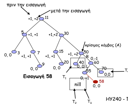
Σχήμα 7.5: Lewis & Denenberg, Data Structures & Their Algorithms, Addison-Wesley, 1991
