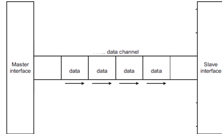
AXI4-Streaming Transfer
