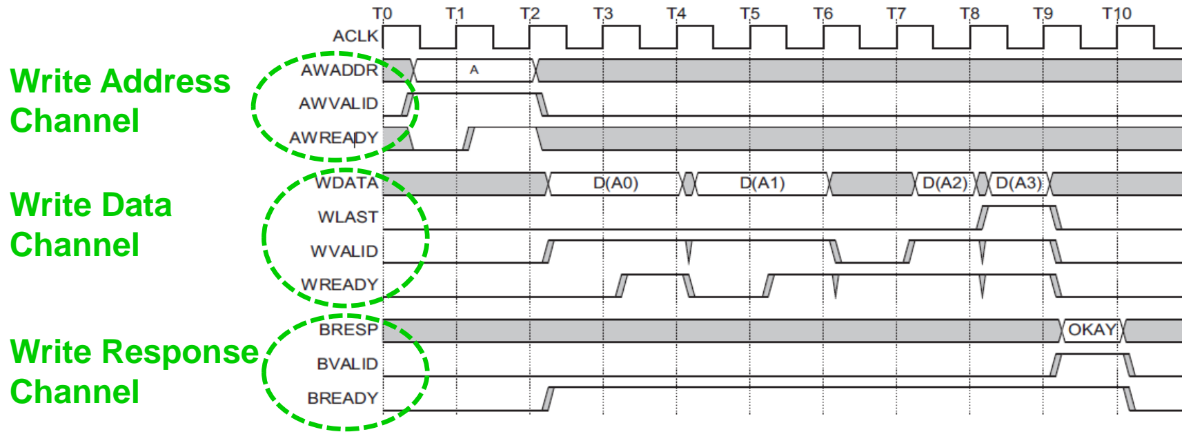
Figure 1-6 Write burst
