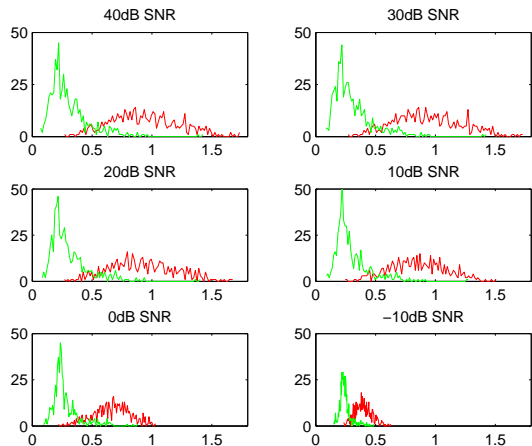
Figure 2: Histogram of relevant response ratios computed on nonspeech (gray/green) and speech examples (black/red).
