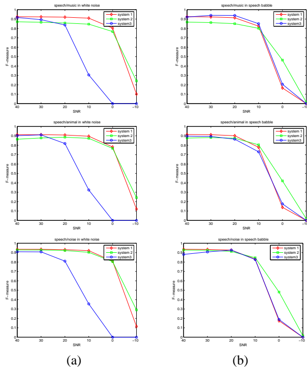
Figure 3: F measure of systems applied to all signal types of the benchmark test : (a) with additive white noise (b) with speech babble.
