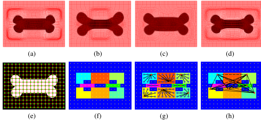
Fig. 1: Synthetic experiment: the upper row shows exemplary deformations and overlaid the corresponding dense displacement fields. The lower row illustrates the clustering (f) and the resulting MRF topology consisting of intra-cluster edges (g) and the fully connected graph on the cluster centers (h).
