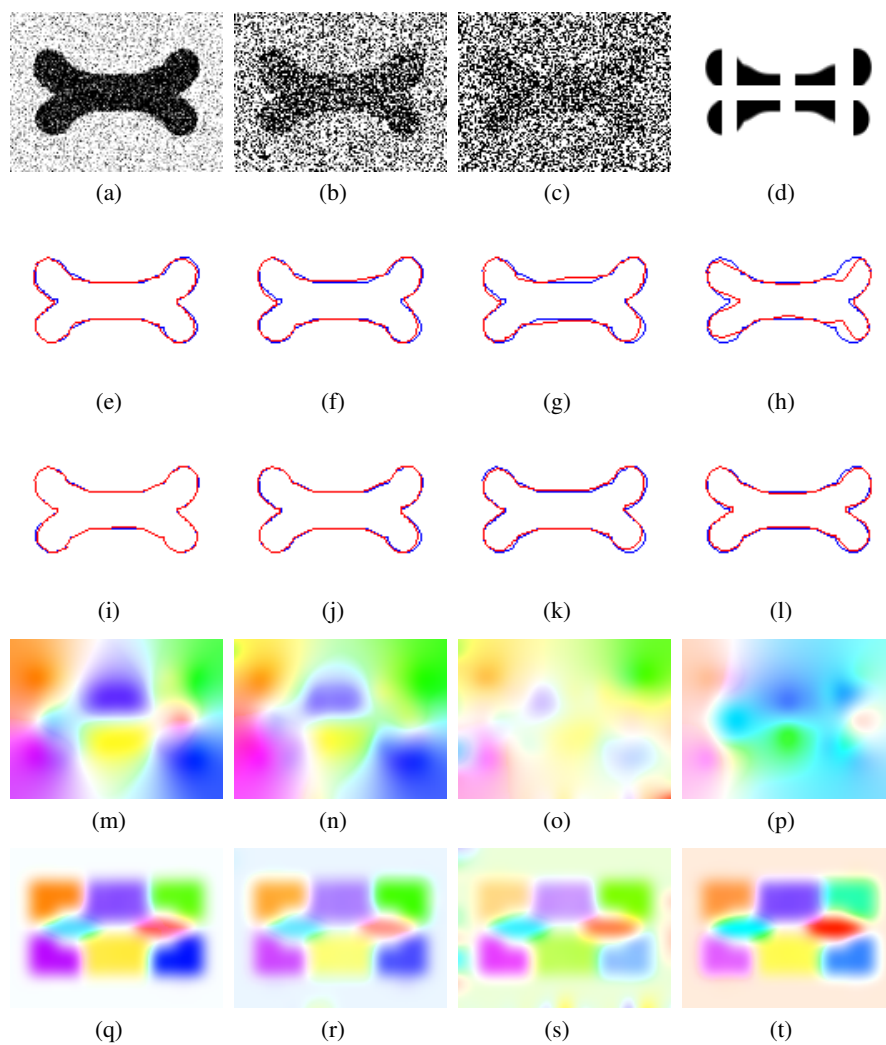
Fig. 3: Synthetic experiment: the first row illustrates exemplary target images with varying amounts of noise and corruption. The second row shows the registration results for the conventional registration while the third row shows the results for using learned priors. The target shape boundary is drawn in blue, the shape boundary of the deformed source image is drawn in red. The initial alignment before registration is illustrated in Fig. 2. The fourth and fifth row show the color encoded displacement fields for both methods. The color represents the angle, the intensity the magnitude of the displacement vectors. Note, how well the clustering topology is reflected in all fields for registration with deformation priors (compare Fig. 1(f)).
