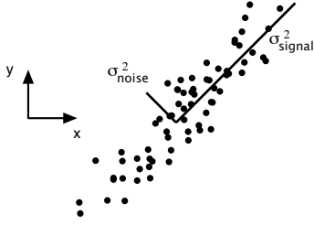
FIG. 2 Simulated data of (x, y) for camera A . The signal and noise variances \sigma_{signal}^2 and \sigma_{noise}^2 are graphically represented by the two lines subtending the cloud of data. Note that the largest direction of variance does not lie along the basis of the recording (x_A, y_A) but rather along the best-fit line.
