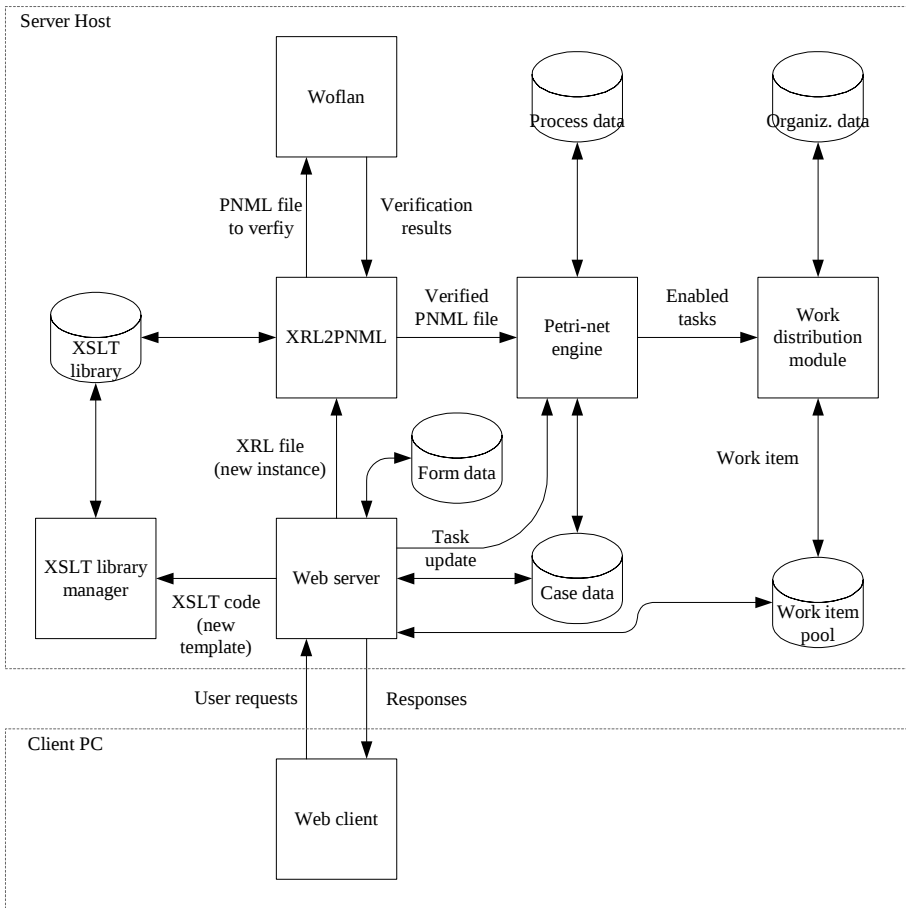
Fig. 2. A detailed architecture for implementing inter-organizational workflows using XRL/Woflan.
