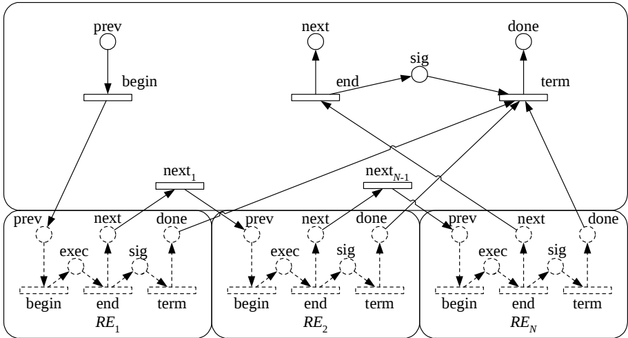
Fig. 1. The Petri-net fragment of the sequence routing element.
