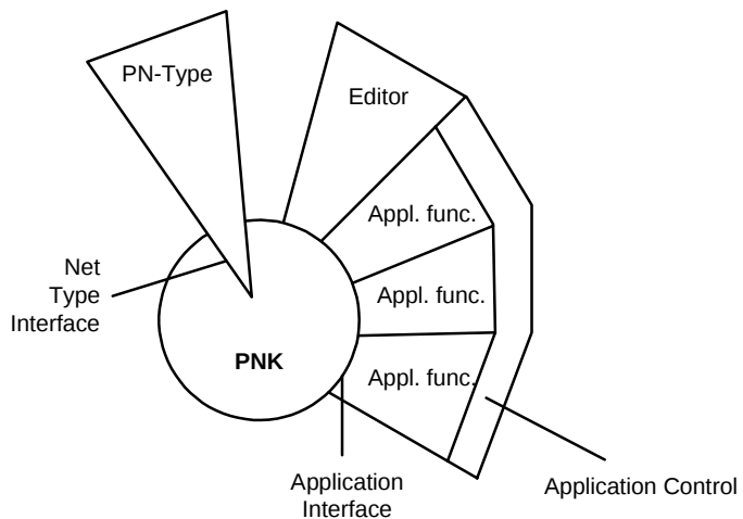
Fig. 4. Conceptual Model of the Petri Net Kernel.
