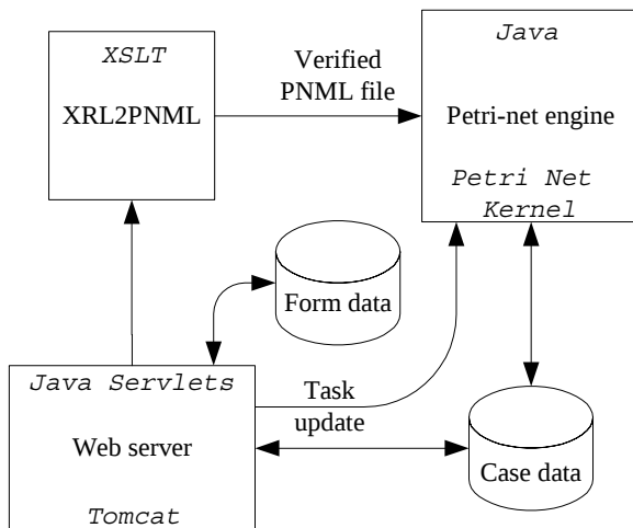
Fig. 3. Choice of Technology for Component Implementation.
