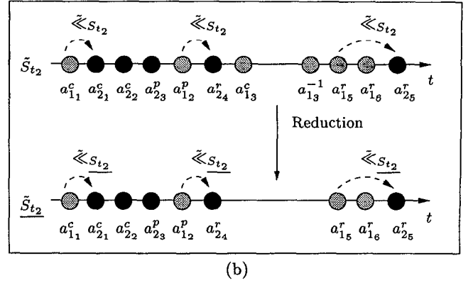
Figure 6: Completed process schedule \tilde{S}_{t_2} (a) and reduced process schedule \tilde{S}_{t_2} (b) of process schedule S_{t_2}
