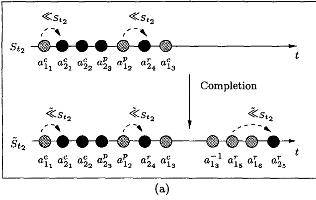
Figure 6: Completed process schedule \tilde{S}_{t_2} (a) and reduced process schedule \tilde{S}_{t_2} (b) of process schedule S_{t_2}
