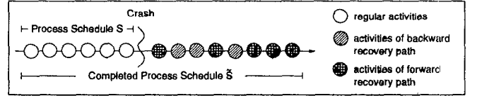
Figure 5: Completion of a process schedule by activities of the backward recovery path and of the forward recovery path of all active processes
