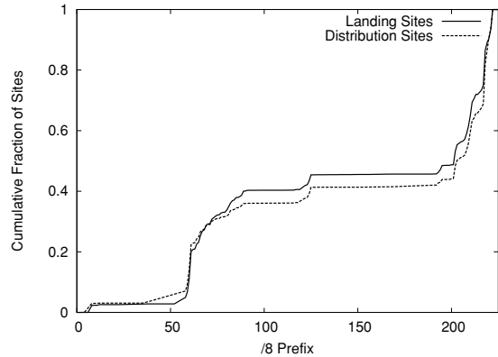
Figure 9: The cumulative fraction of malware distribution sites over the /8 IP prefix space.
