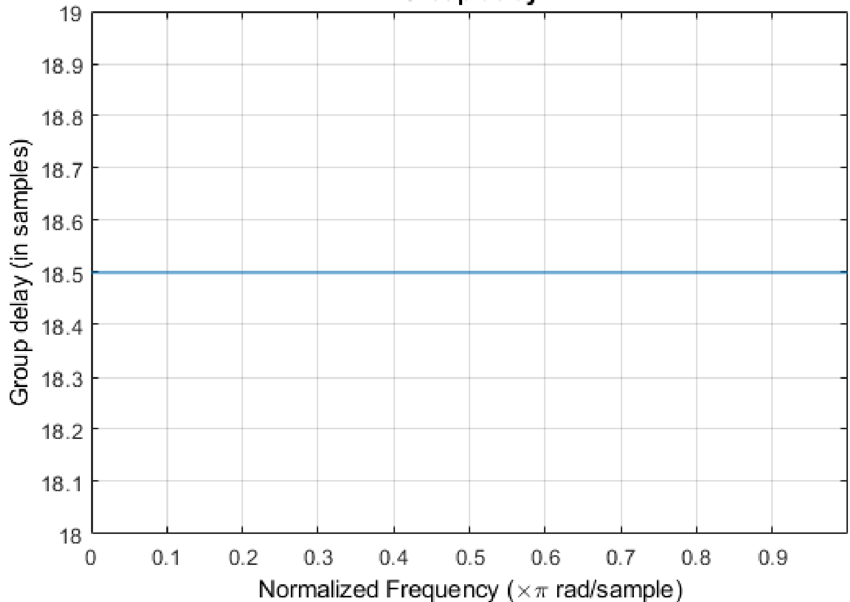
Group delay
