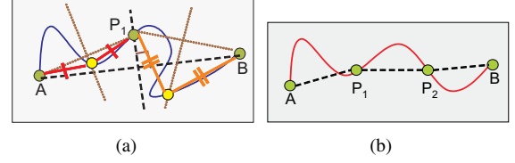
Fig. 1. (a) The segment bisector based method has been inductively applied for N = 4 . The corresponding line segments are not necessary equal. (b) A curve equipartition example for N = 3 , |AP_1| = |P_1P_2| = |P_2B| under Euclidean distance metric.
