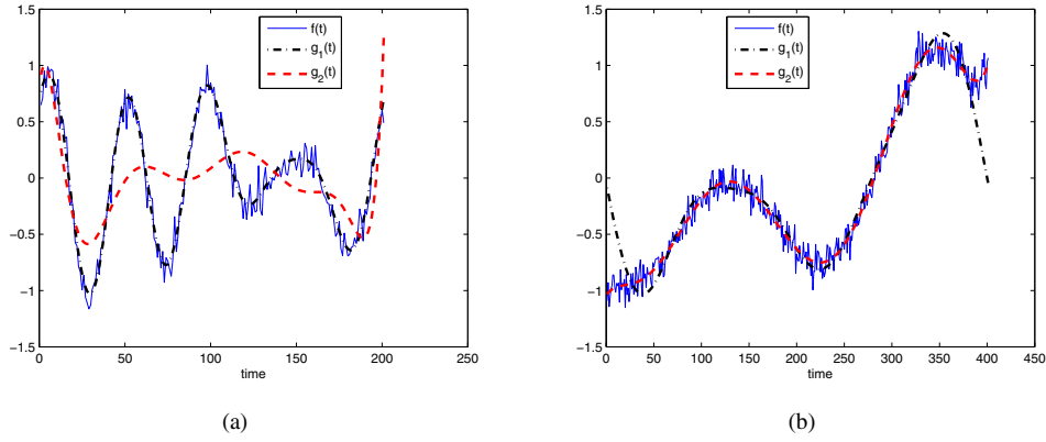
Fig. 2. The given synthetic signals (blue line) are approximated by g_1(t) and g_2(t) with S = 5 . (a) d_1(0, 200) = 0.0063 and d_2(0, 200) = 0.2082 . (b) d_1(0, 400) = 0.0086 and d_2(0, 400) = 0.0465
