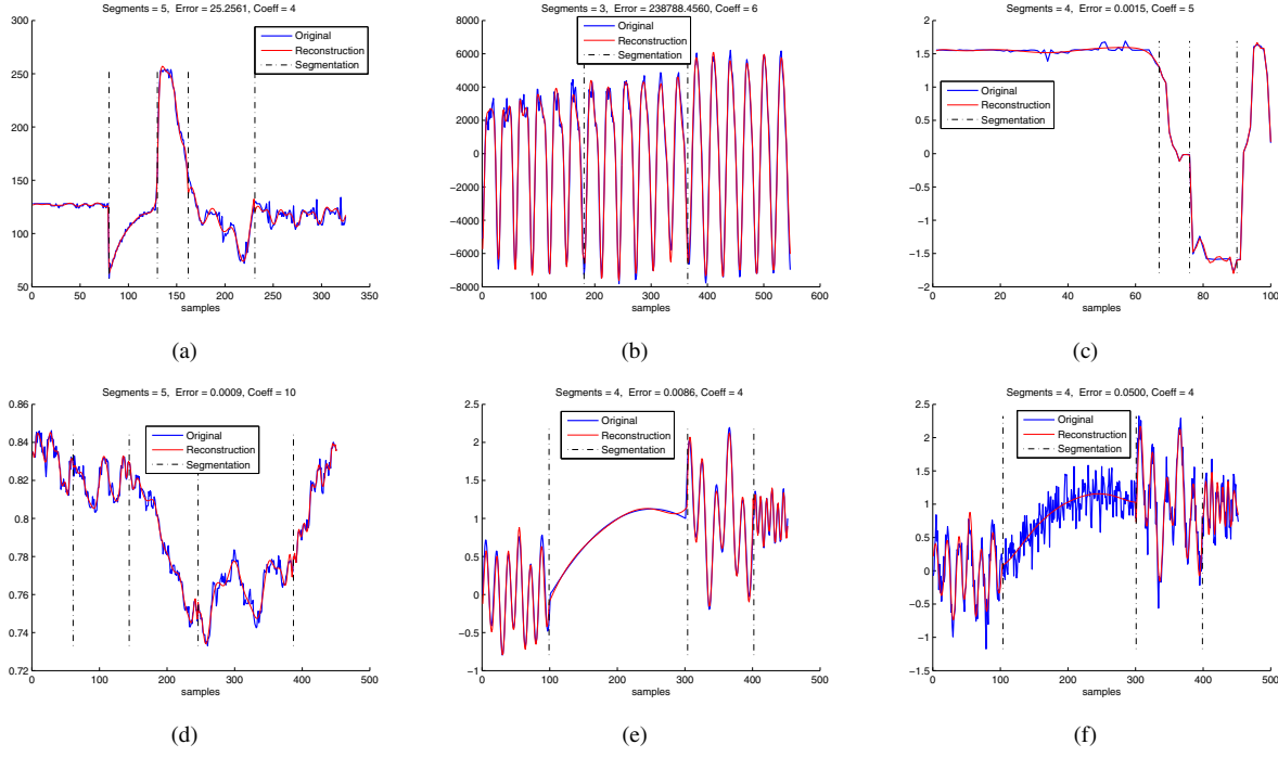
Fig. 3. Original signal (blue curves) and segmentation (black dotted lines) - modelling (red curves) results of the proposed method on: (a) electrocardiogram (ECG), (b) speech signal, (c) human major axis angle signal, (d) EURO-USD exchange rate, (e) synthetic signal, (f) synthetic signal with noise.
