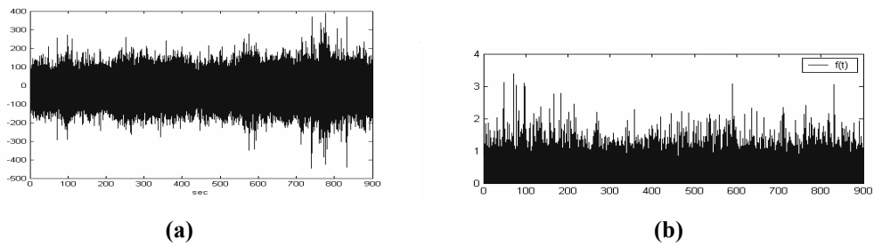
Figure 8 (a) an other example of noise recording on z component, (b) the f(t) function of the previous noise recording.
