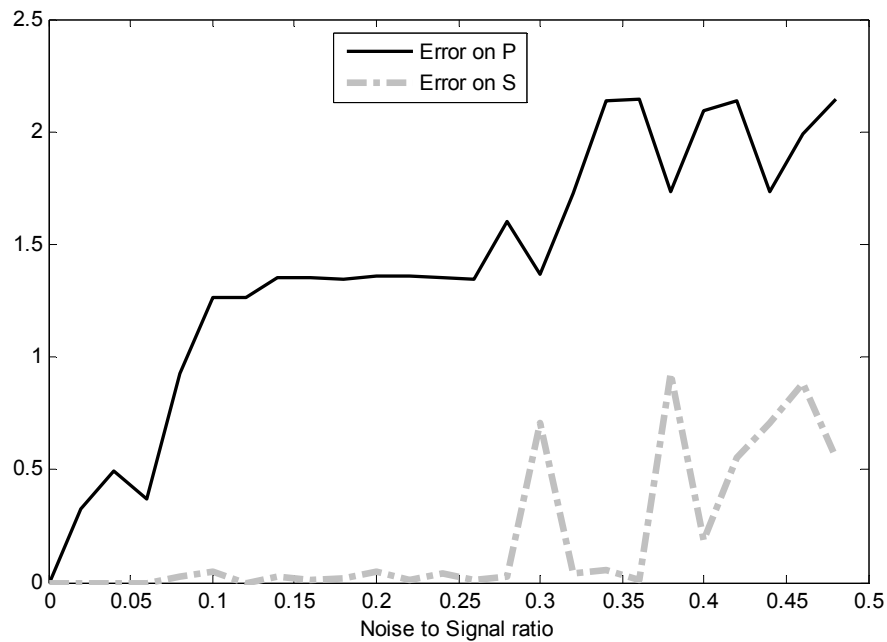
Figure 9 The P and S detection error (in seconds) in respect to noise to signal ratio for the 8th January 2006 (11:35:09.895 UTC, mb=6.7, CMT Harvard routine analysis) earthquake z signal.
