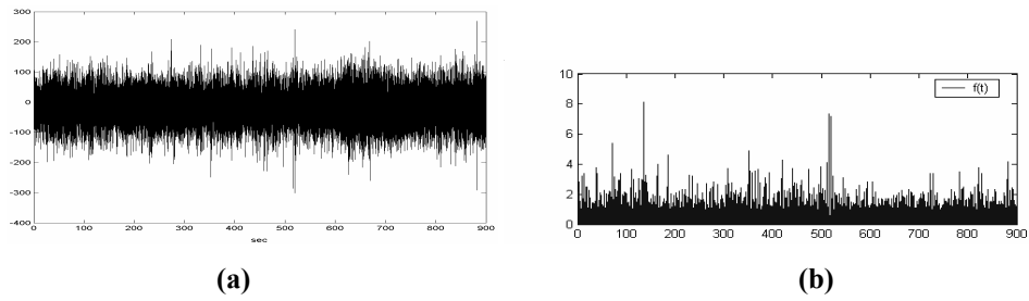
Figure 7(a) noise recording on z component, (b) the f(t) function of the previous noise recording.
