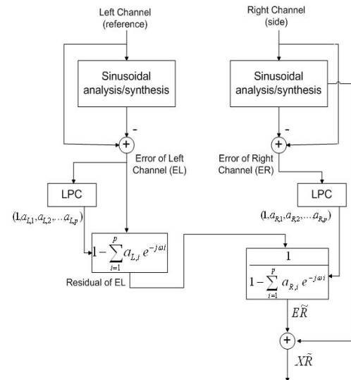
Fig. 1: Noise transplantation. The LPC residual of the reference signal's noise component is filtered by the side signal's noise envelope and added to its sinusoidal component.
