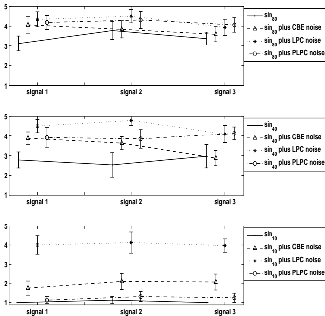
Fig. 2: Results from the quality rating DCR listening tests corresponding to sinusoidal modeling with (a) 80 sinusoids per frame (upper), (b) 40 sinusoids per frame (middle), and (c) 10 sinusoids per frame (lower).
