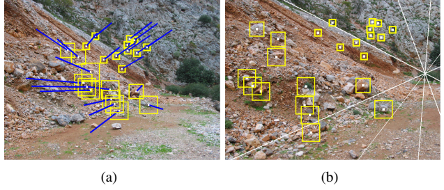
Fig. 2: (a) Image I_k along with computed optical flow vectors (blue segments) for all points marked white. (b) Image I_{k+1} along with matching points (also marked white) for all marked points of (a). A few epipolar lines are also shown. In both images, the yellow square around a point is analogous to the point's estimated scale factor (10 scales S = \{1, 0.9^{-1}, \dots, 0.1^{-1}\} have been used).
